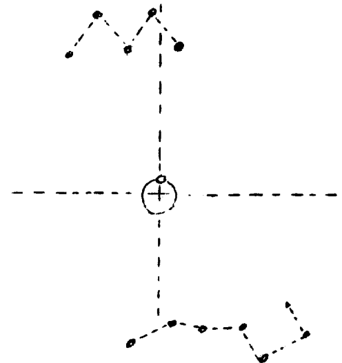
Polaris 1^{\circ} above the Pole and on the meridian
