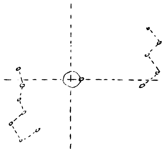
Polaris at the same altitude as the Pole but 1^{\circ} East of the meridian
