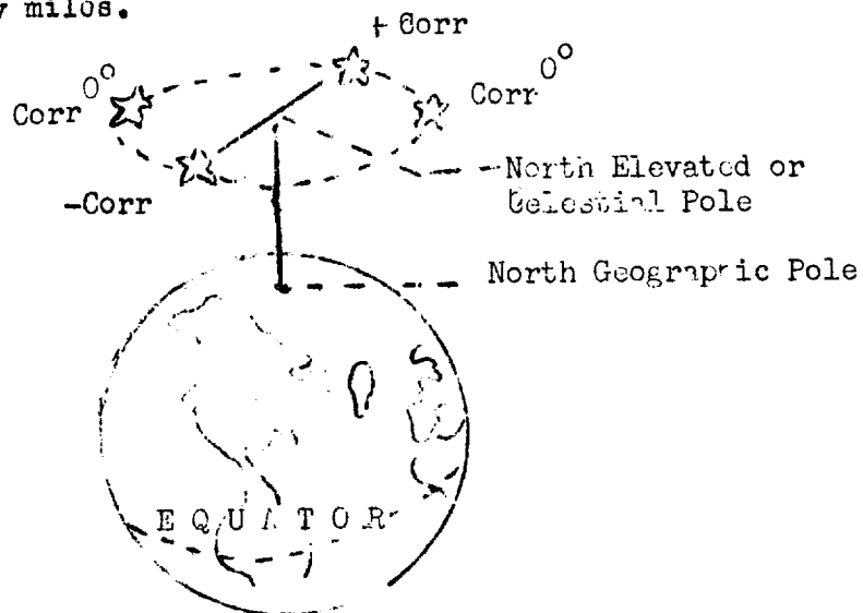
North Elevated Pole
